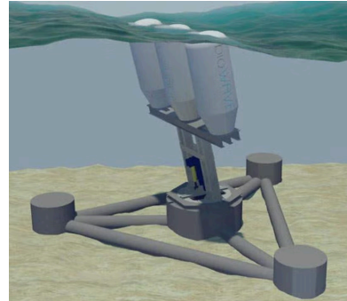
BioPower Systems Pty Ltd. bioWAVE on the sea floor.
